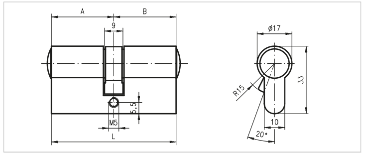
Plan technique
